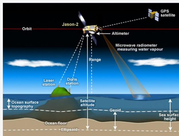
Figure 2: The measurement of sea surface height from Jason-2 with respect to ellipsoid [32].
