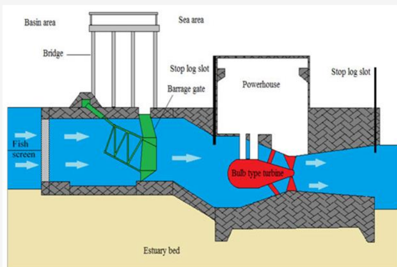
Figure 7: The cross-section of Kuching Barrage with the proposed of bulb type turbine for power generation during the ebb tide [44]
