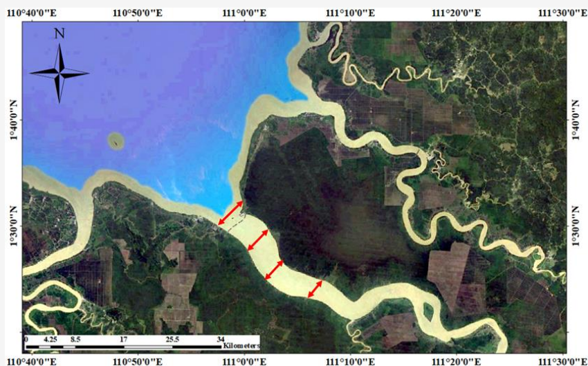
Figure 4: Estuary width on the river near the Maludam coastlines of Sarawak (retrieved from Google Earth). The width of the estuary decreases (red arrows) towards the land and creates funneling and shoaling activities, which affect the dynamic of the tidal range
