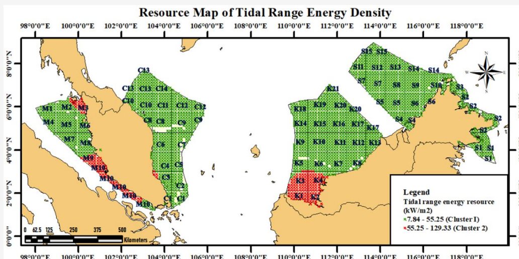
Figure 5: Resource map for tidal range energy in EEZ ( \text{kW}/\text{m}^2 )
