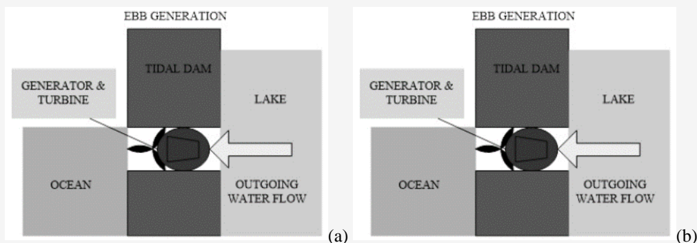
Figure 6: Tidal barrage operation for one-way power generation during ebb tide (a) and during flood tide (b) [41]
