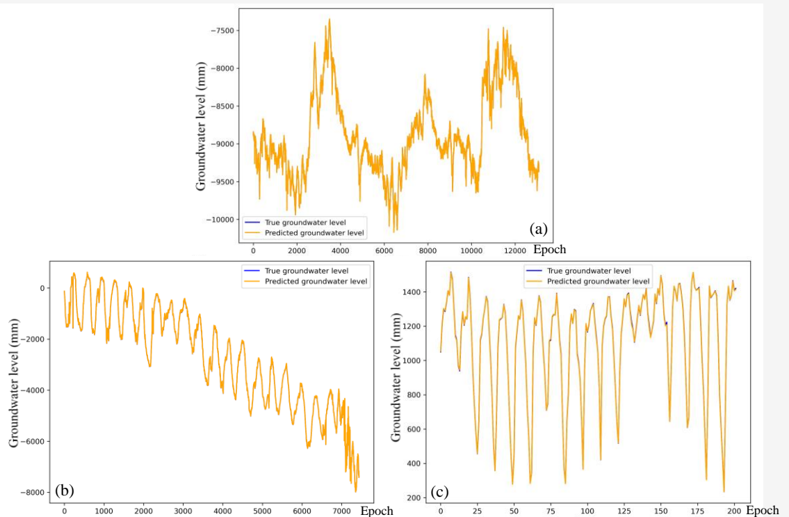
Figure 3: SimpleRNN predicted and actual groundwater level at observation stations: (a) Q55M1 (b) Q808010 (c) Q40101T
